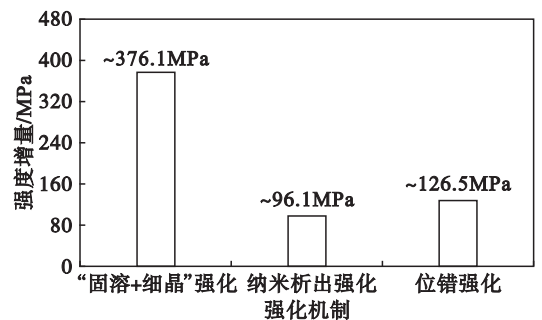
图 5 不同强化机制对材料强度的贡献值 Fig. 5 Strengthening contribution induced by different strengthening mechanisms
